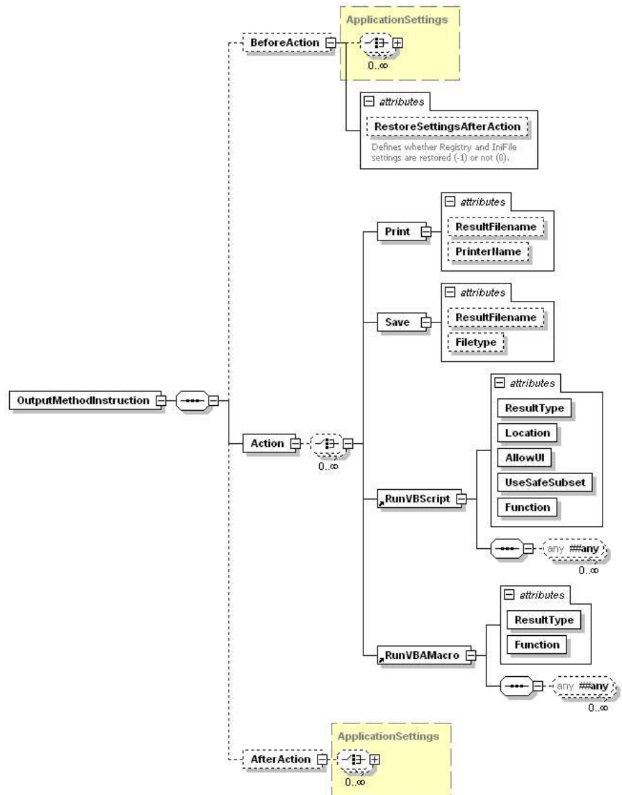
Figure 2: officatwork OOMI-XML Structure
