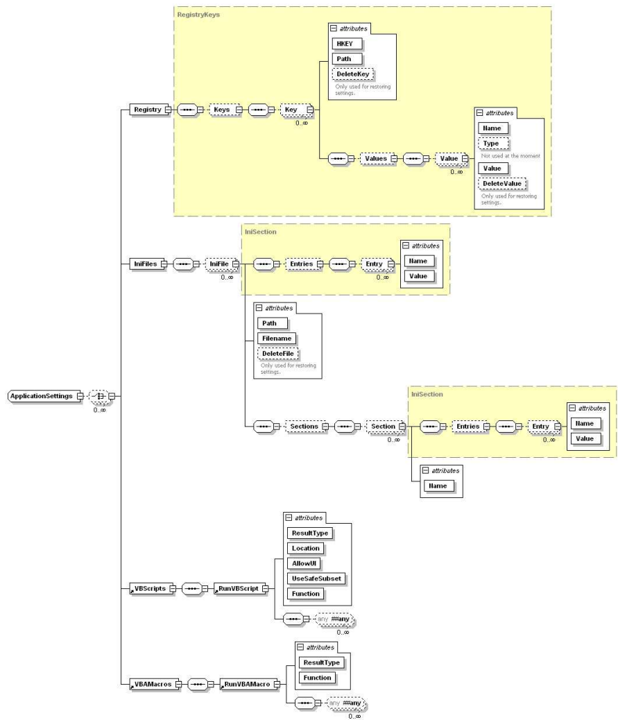
Figure 3: officeatwork OOMI-XML structure, ApplicationSettings
